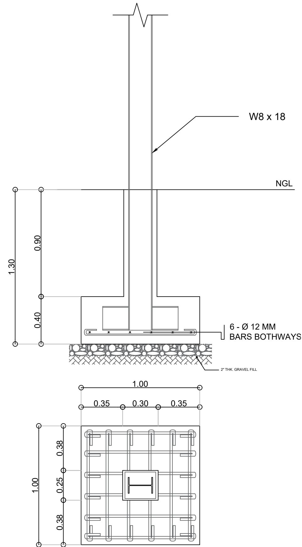
1 COLUMN / FOOTING DETAIL SCALE 1 : 30 M.
