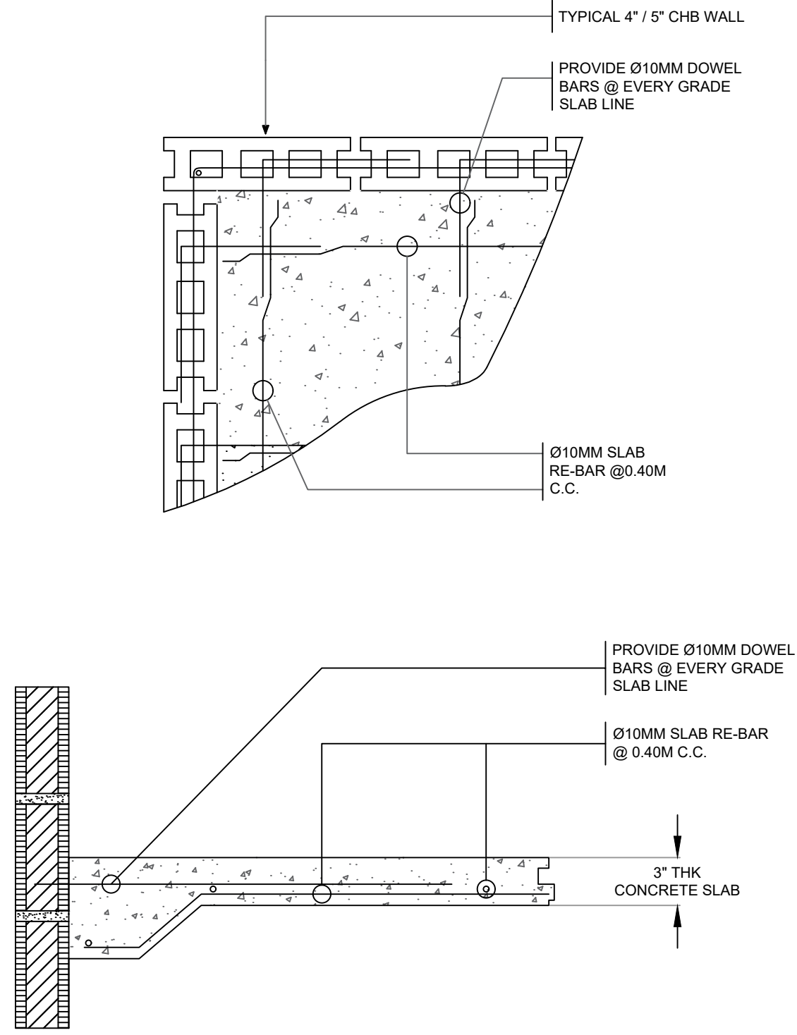
3 SLAB ON GRADE DETAIL SCALE 1 : 10 M.
