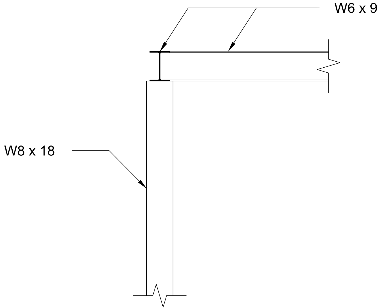
2 COLUMN-BEAM CONNECTION (WELDED) SCALE 1 : 10 M.
