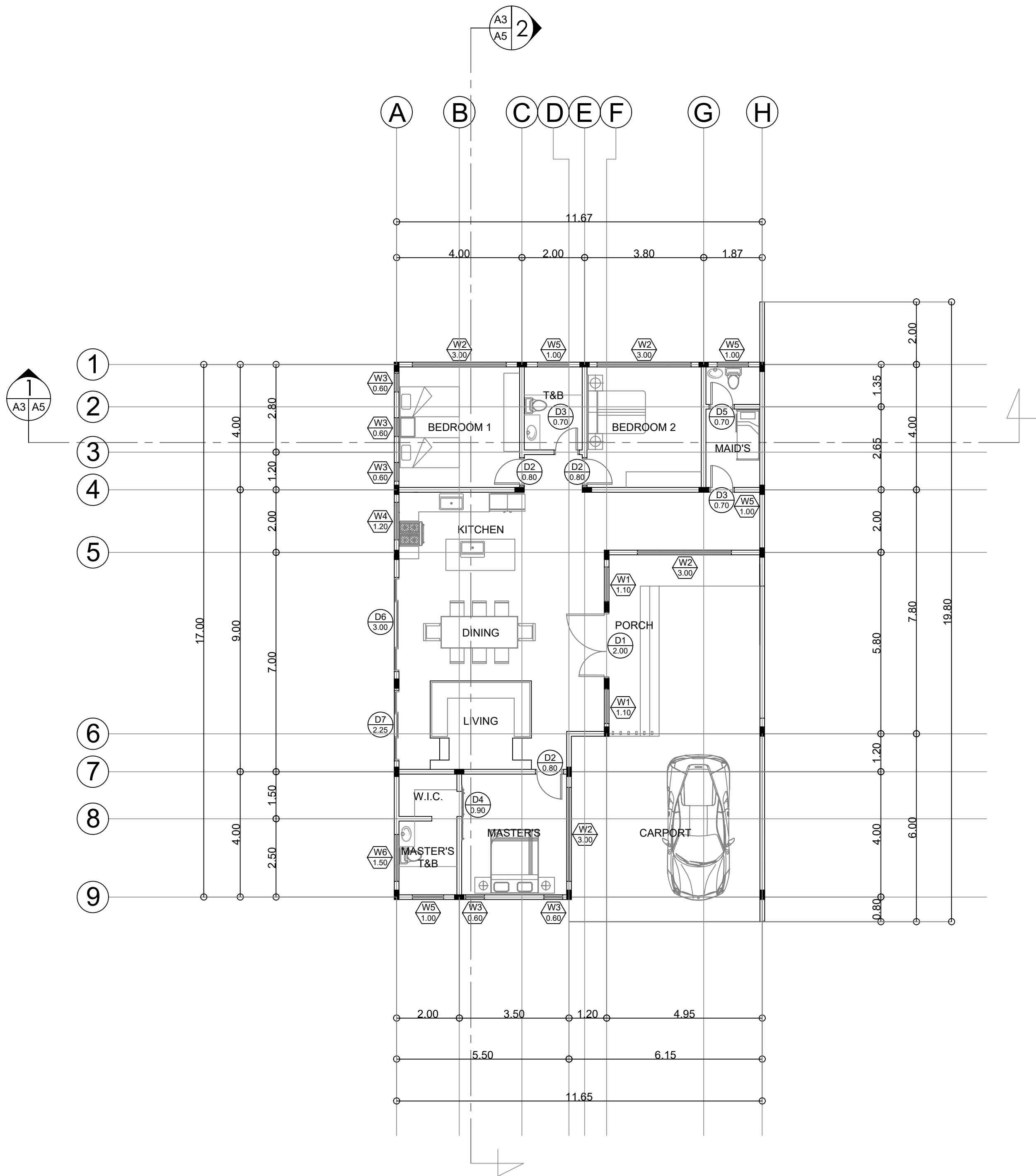
1 GROUND FLOOR PLAN A2 A5 SCALE 1 : 100 M.
