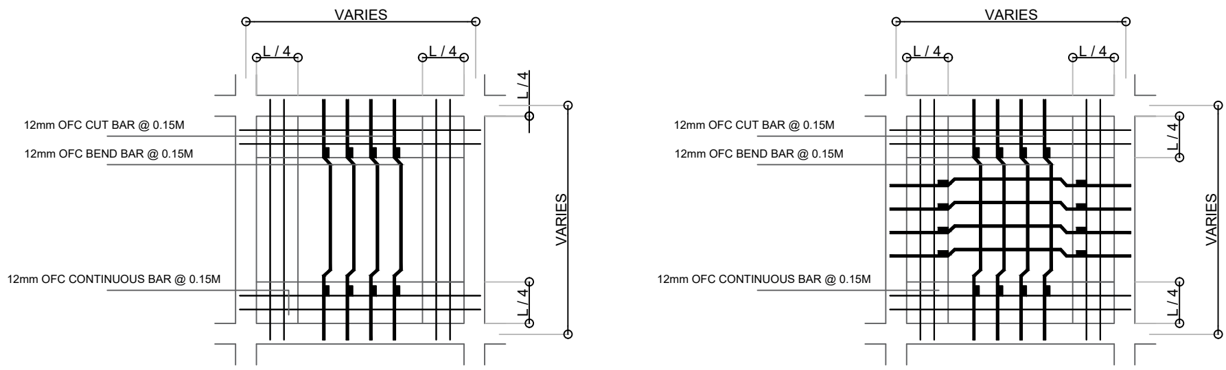
6 SLAB ON GRADE DETAIL SCALE 1 : 25 M.
